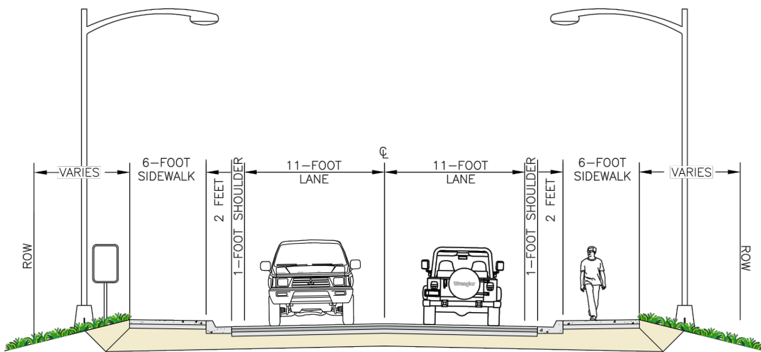
TYPICAL SECTION, BLOCK 1
