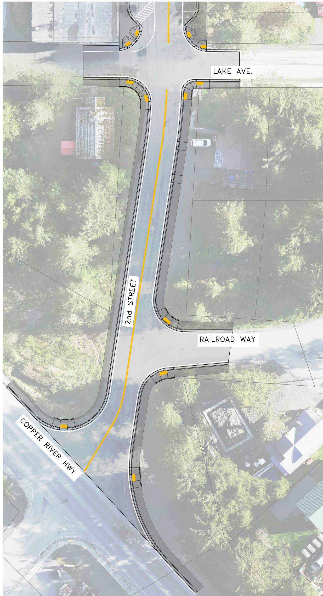
PLAN VIEW
